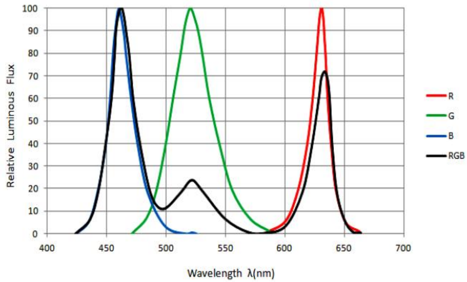
Figure 1a. Typical normalized power vs. wavelength for at test current, T_j = 25^\circ \text{C} .
