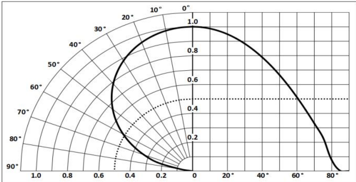
Typical radiation pattern for at test current(350mA), Tj =25°C
