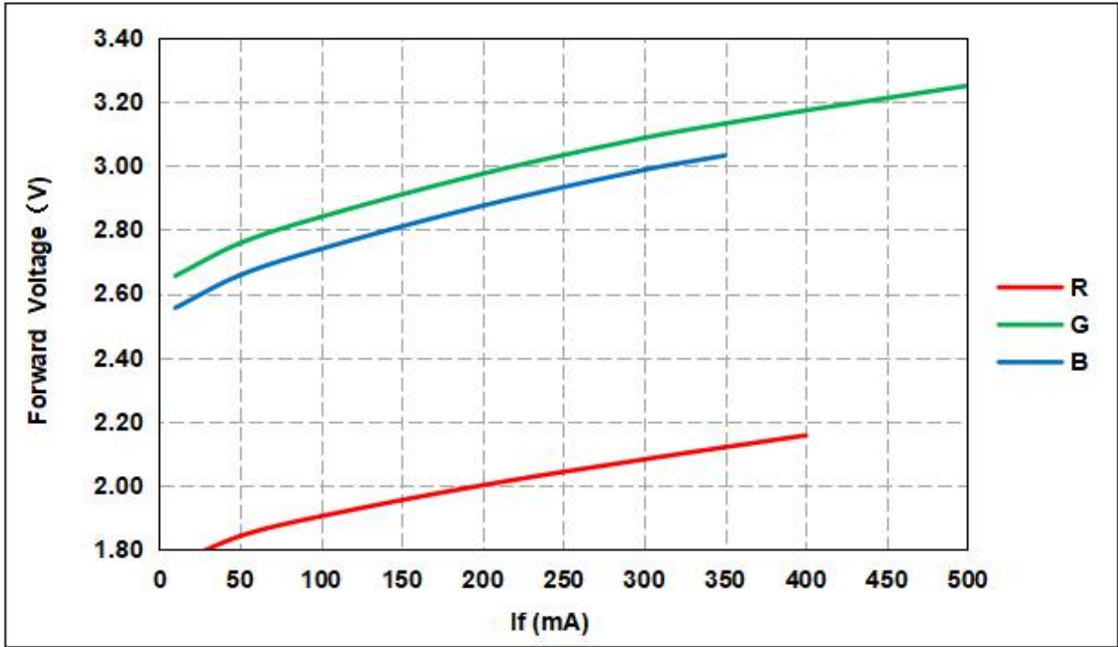
Forward Voltage VS Forward Current (IF=350mA, 25°C)
