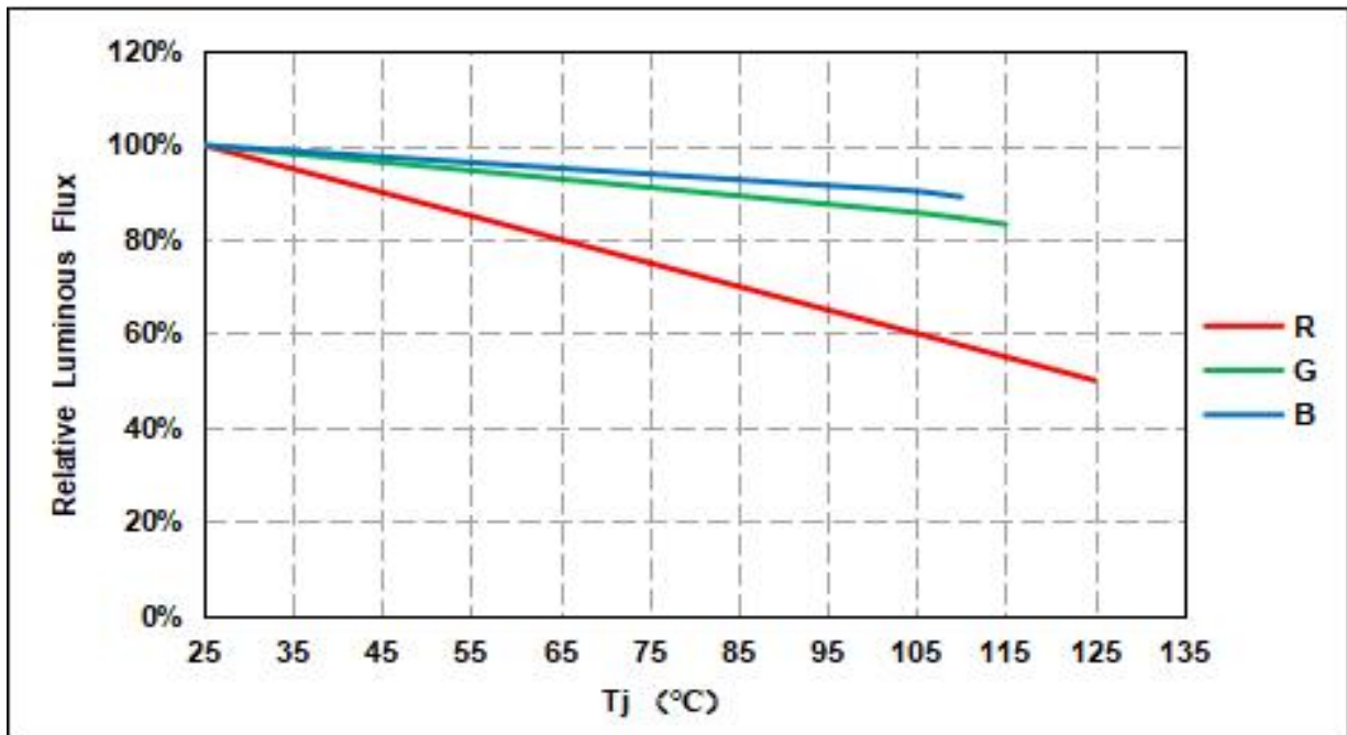
Relative Luminous Intensity VS Junction Temperature (IF=350mA, 25°C)
